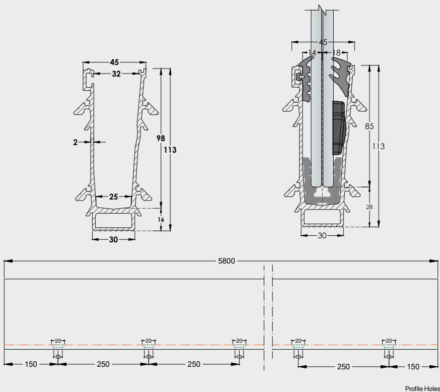
Profile Holes
