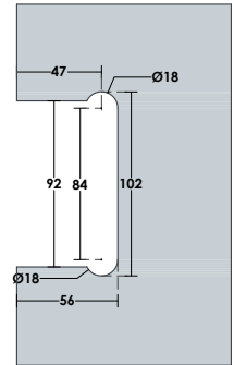
Glass Cut
