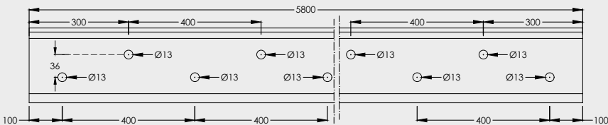
Profile Holes
