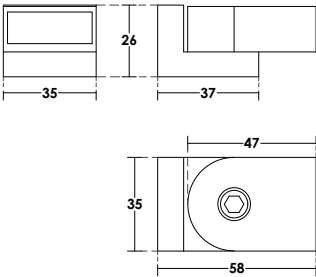
PCA-HL44 Adjustable Wall - Track Holder Stainless Steel 304 | Material Satin, Polished, Black Anodize | Finish
