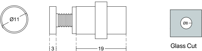
PCA-HR06 Self Holder 5-10mm | Glass Thickness Zinc Alloy | Material Satin, Polished | Finish
