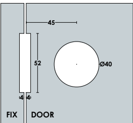
PCA-BL13 Magnetic Door Lock 10-12mm | Glass Thickness Stainless Steel 304 | Material Satin | Finish
