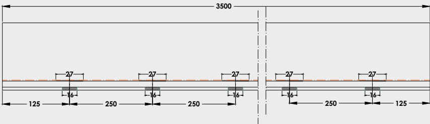
Profile Holes
