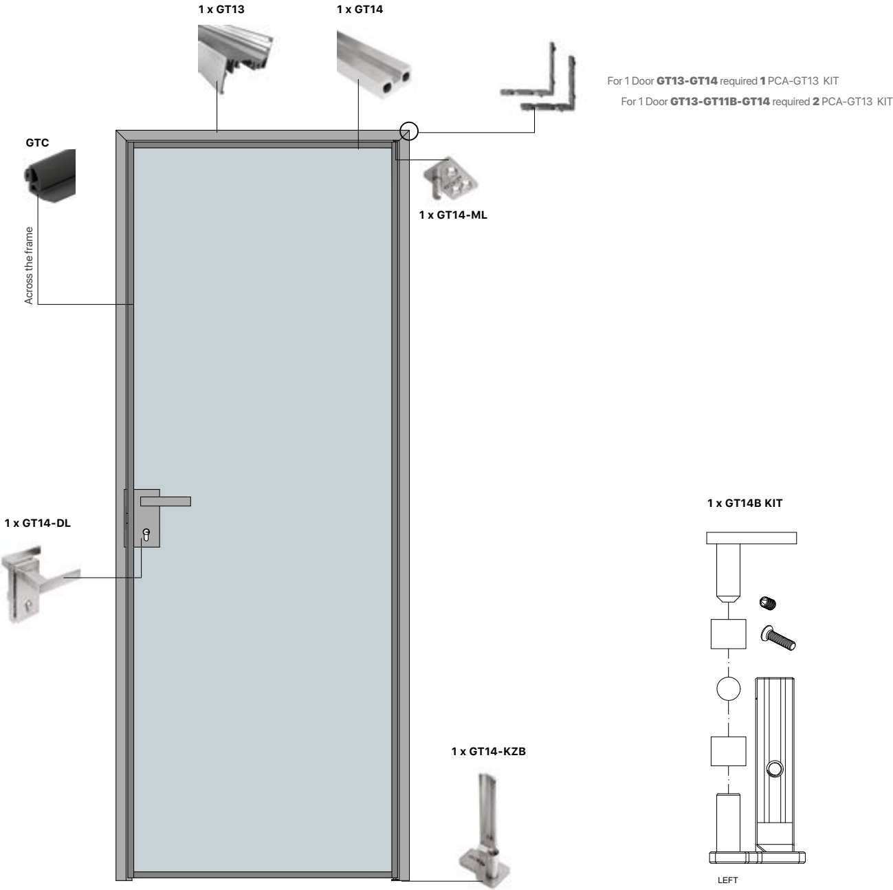
GT13 Frame | GT14 Door Section Details
