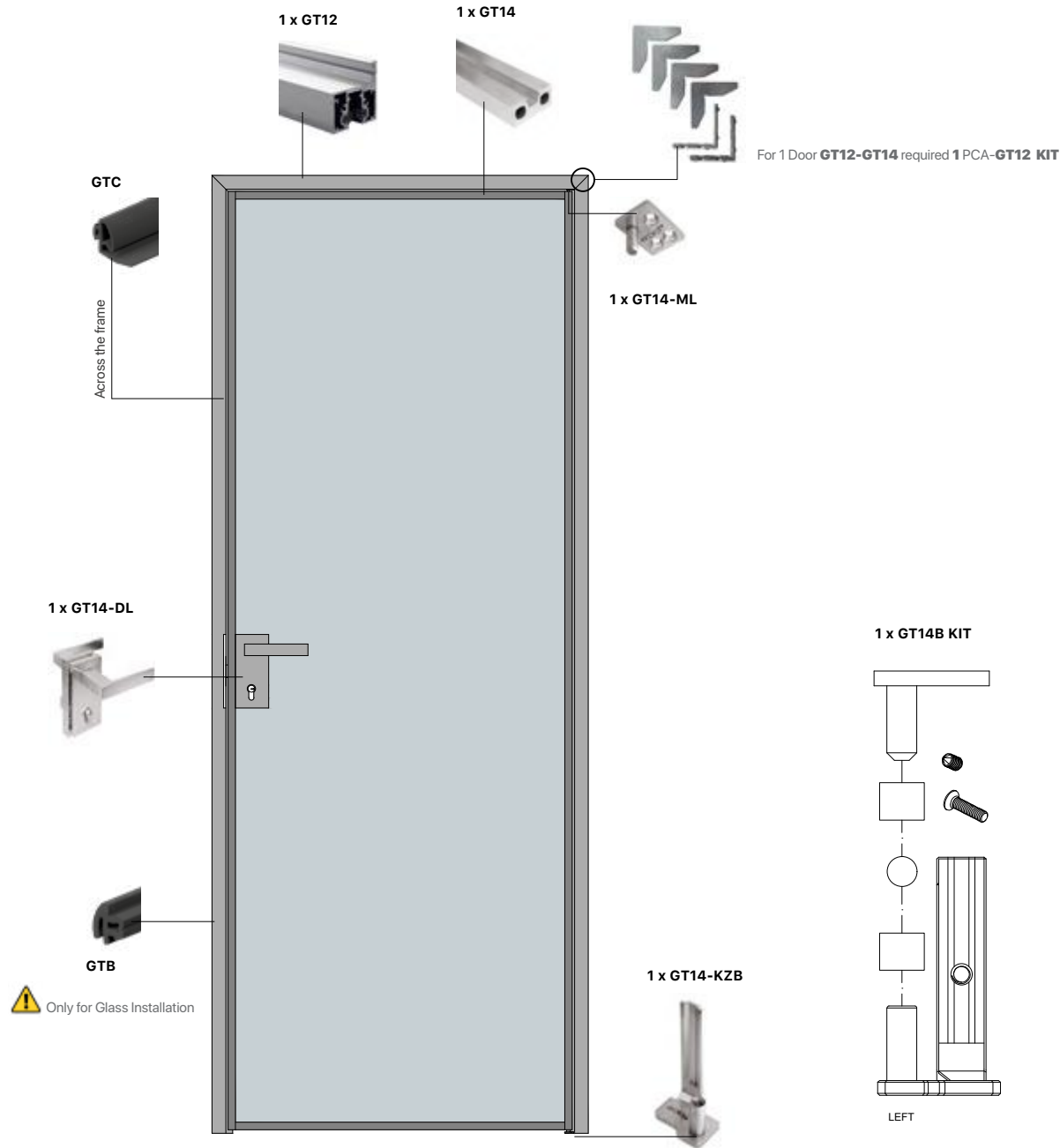
GT12 Frame | GT14 Door Section Details
