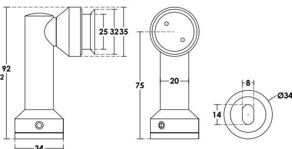
Ø 26-32 Glass Hole
