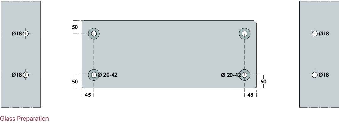
Glass Preparation
