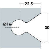
Glass Cut
