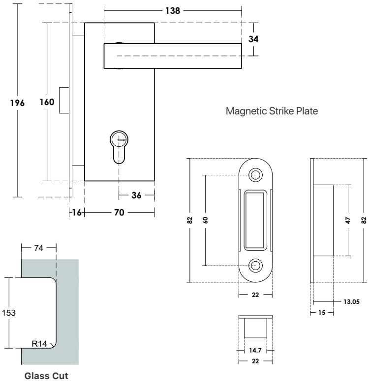
Door Lock for GT14
