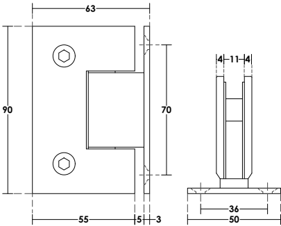
PCA-SH31 Glass - Wall Hinge 10mm | Glass Thickness 40 kg | Max. Weight Zinc Alloy,Stainless Steel 304| Material Satin, Polished, Black Anodize | Finish
