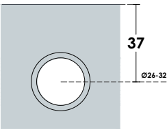
Glass Cut
