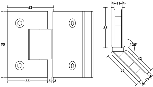
PCA-SH35 135° Glass - Glass Hinge 10mm | Glass Thickness 40 kg | Max. Weight Zinc Alloy,Stainless Steel 304| Material Satin, Polished, Black Anodize | Finish
