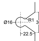
Glass Cut
