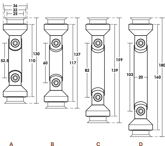
PCA-FC01 Facade Glass - Glass Clamp 10-12mm | Glass Thickness 50 kg | Max. Weight Stainless Steel 304 | Material Satin | Finish
