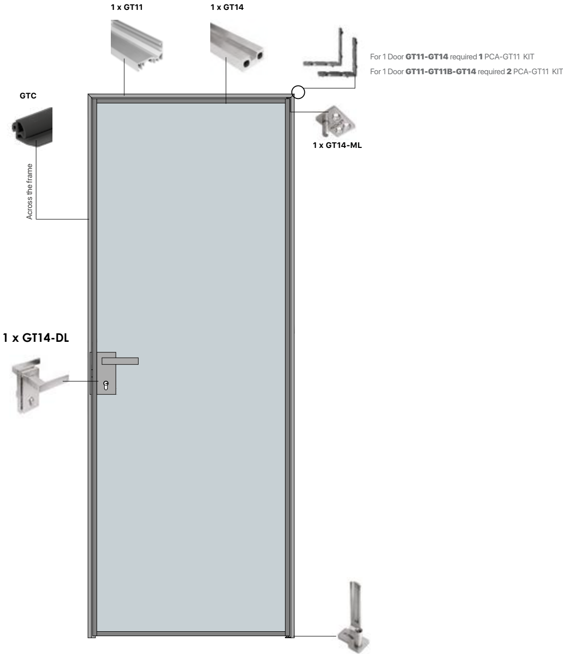
GT11|GT11-GT11B Frame | GT14 Door Section Details
