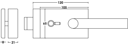
PCA-DL09A DL04 Strike Plate Aluminium| Material Natural Anodize,Satin, Black Anodize | Finish
