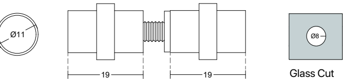
PCA-HR07 Self Holder 5-10mm | Glass Thickness Zinc Alloy | Material Satin, Polished | Finish
