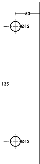
Glass Cut
