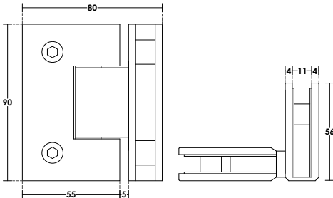
PCA-SH37 90° Glass - Glass Hinge 10mm | Glass Thickness 40 kg | Max. Weight Zinc Alloy,Stainless Steel 304| Material Satin, Polished, Black Anodize | Finish
