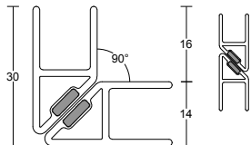
PCA-S09 Waterproof Sealant 90° Magnet 8,10mm | Glass Thickness 300,220cm | Length PVC | Material
