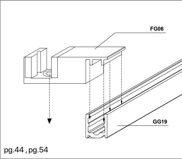
U - profile option
