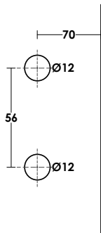
Glass Cut
