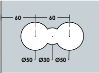
Glass Cut
