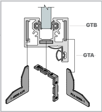
GT12 CORNER DETAIL For 1 Door required 1 PCA-GT12 KIT
