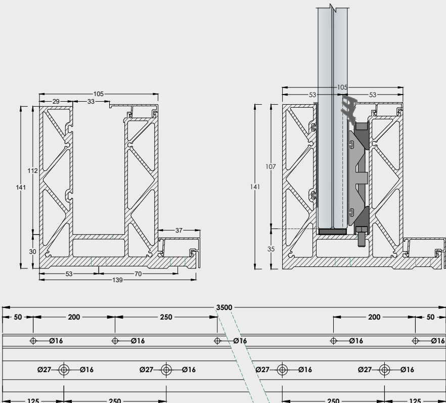
Profile Holes
