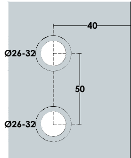
Glass Cut
