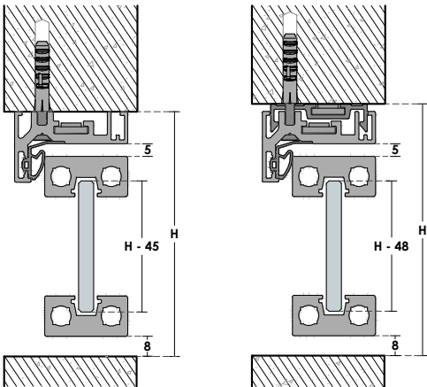
GT11|GT11-GT11B Frame | GT14 Door Section Details
