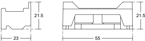
Glass Support | 2PCS / Panel
