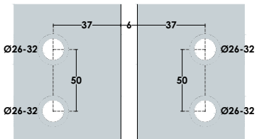
Glass Cut
