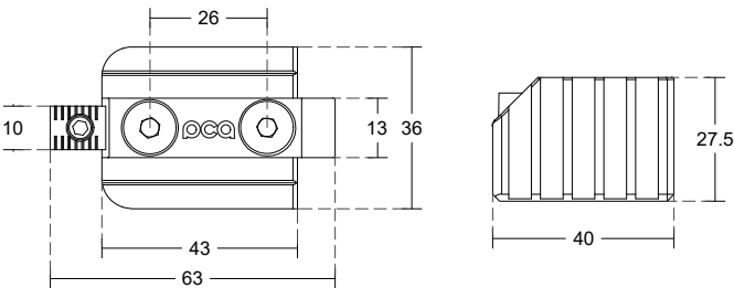
GG08-U Connection
