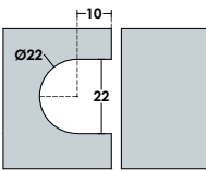
Glass Cut
