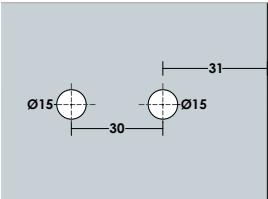
Glass Cut
