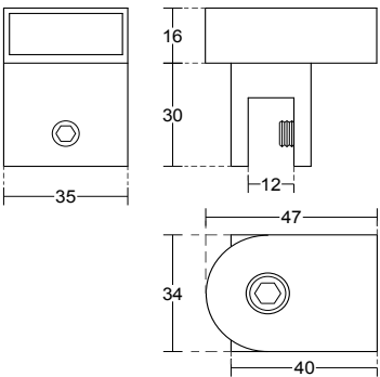
PCA-HL47 Adjustable Glass - Track Holder 10mm | Glass Thickness Stainless Steel 304 | Material Satin, Polished, Black Anodize | Finish
