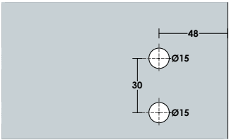
Glass Cut
