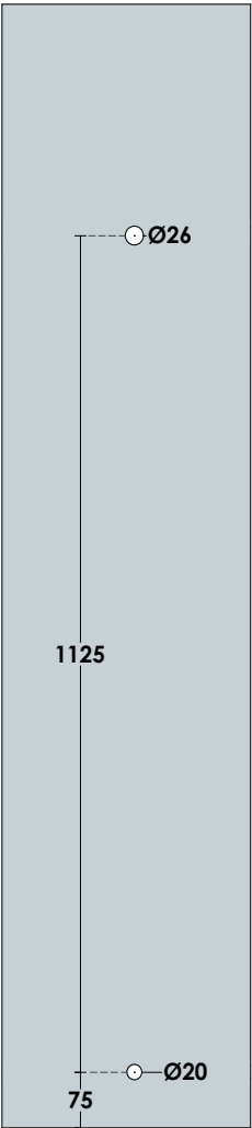
Glass Cut
