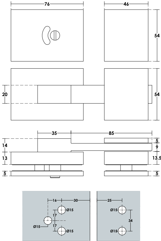
Glass Cut
