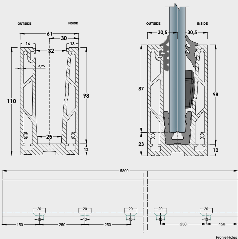
Profile Holes
