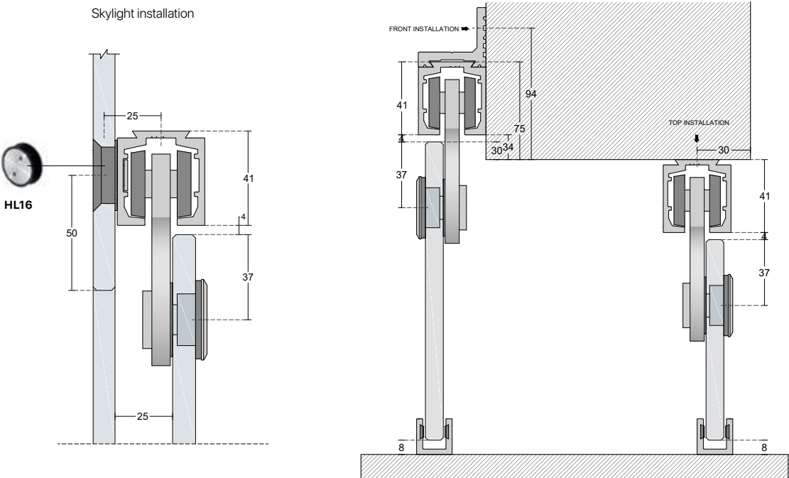
Skylight installation
