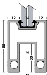
12mm glass S38 polycarbonate
