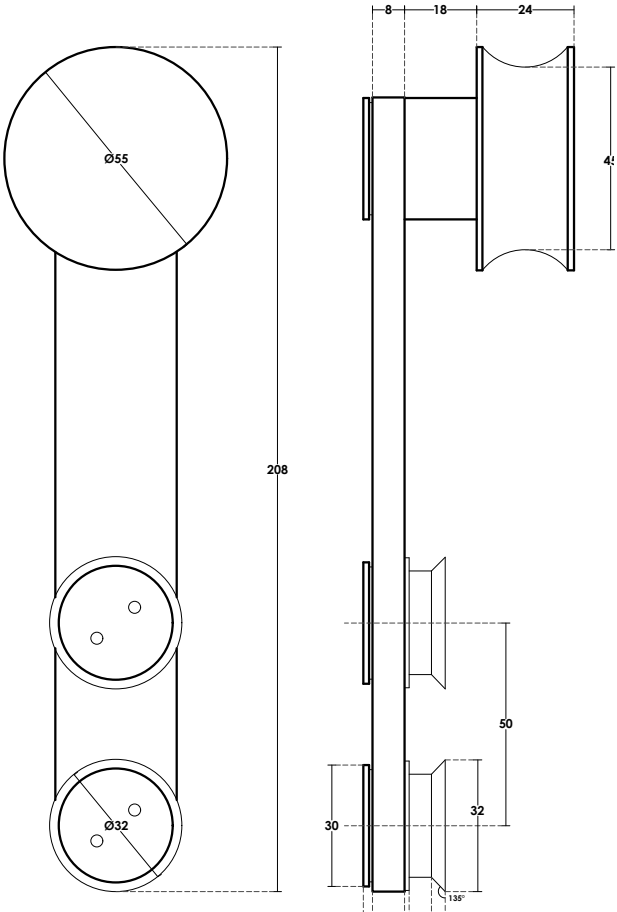
Up side of Glass COUNTER SUNK HOLES
