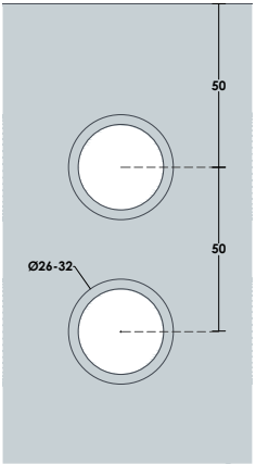
Up side of Glass COUNTER SUNK HOLES
