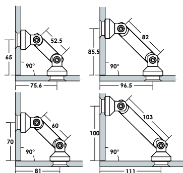
Ø 26-32 Glass Hole
