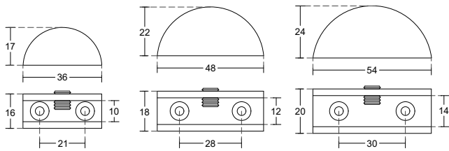
PCA-HR01 | HR02 | HR03 Self Holder 5-10mm | Glass Thickness Zinc Alloy | Material Satin, Polished | Finish
