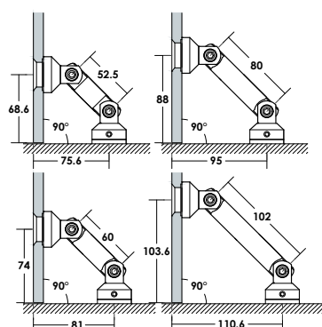
Ø 26-32 Glass Hole
