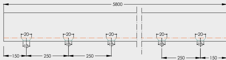
Profile Holes
