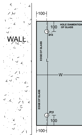
PCA-HL30 Wall- Glass Fitting 10,76-21,52 | Glass Thickness 80 kg | Weight Stainless Steel 304 | Material Satin | Finish
