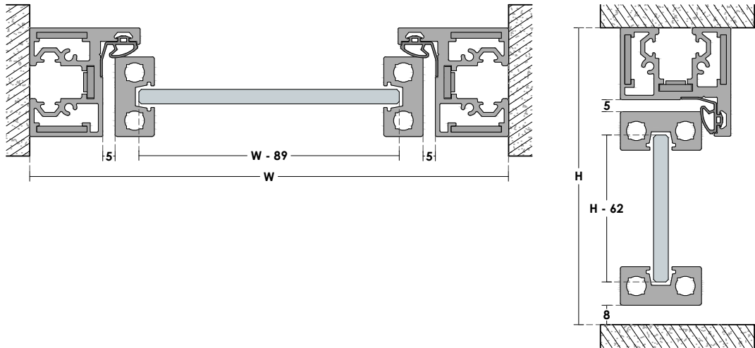
GT12 Frame | GT14 Door Section Details
