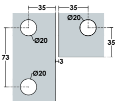
Glass Cut
