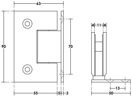
PCA-SH33 Glass - Wall Hinge 10mm | Glass Thickness 40 kg | Max. Weight Zinc Alloy,Stainless Steel 304| Material Satin, Polished, Black Anodize | Finish
