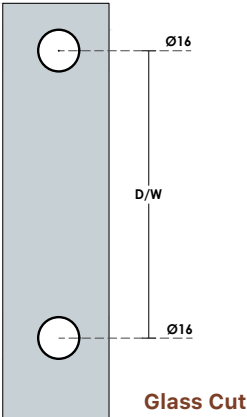
Glass Cut
