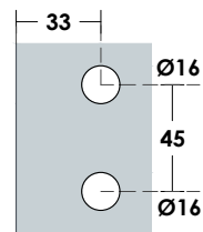
Glass Cut
