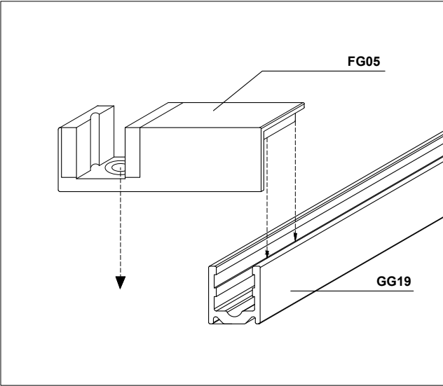
Waterproof bottom track option
