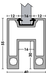
10mm glass S38 polycarbonate
