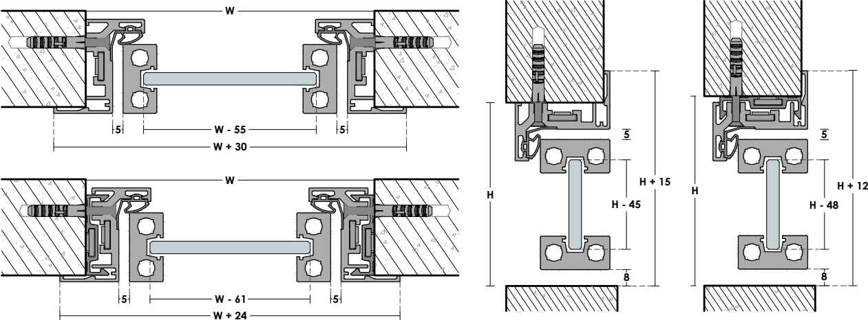
GT13 Frame | GT14 Door Section Details
