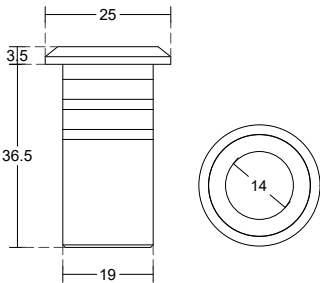
PCA-KP01 Floor Socket Stainless Steel 304 | Material Satin | Finish
