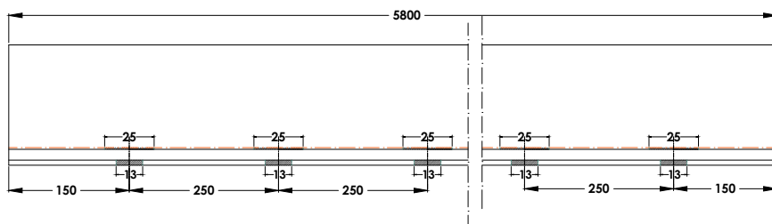
Profile Holes
