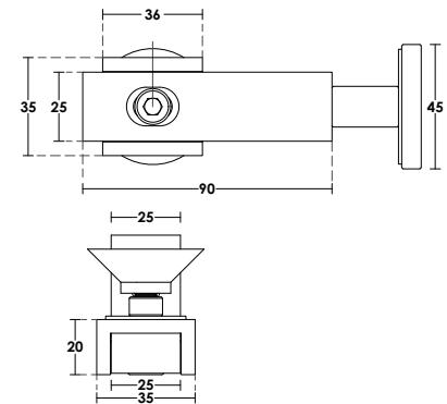
PCA-FC11 Glass Staircase Fitting 560 gr | Weight 50kg | Max Weight 16-30mm | Glass Thickness Stainless Steel 304 | Material Satin | Finish
