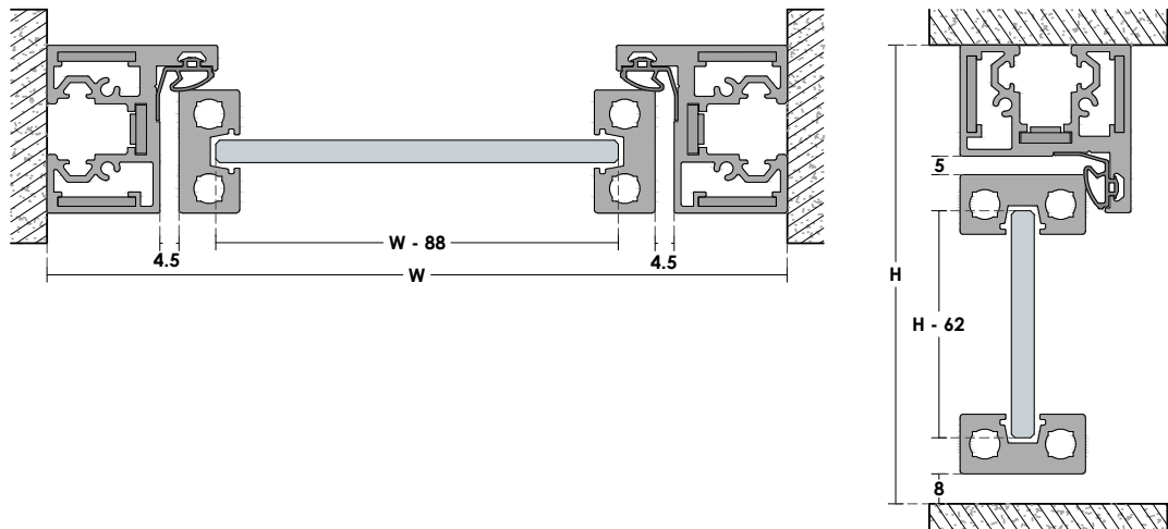
GT12 Frame | GT14 Door Section Details
